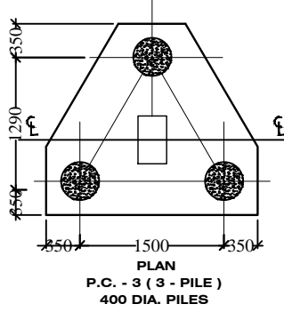
COLUMN LAYOUT BUILT UP AREA - 1324.40SQ.M
